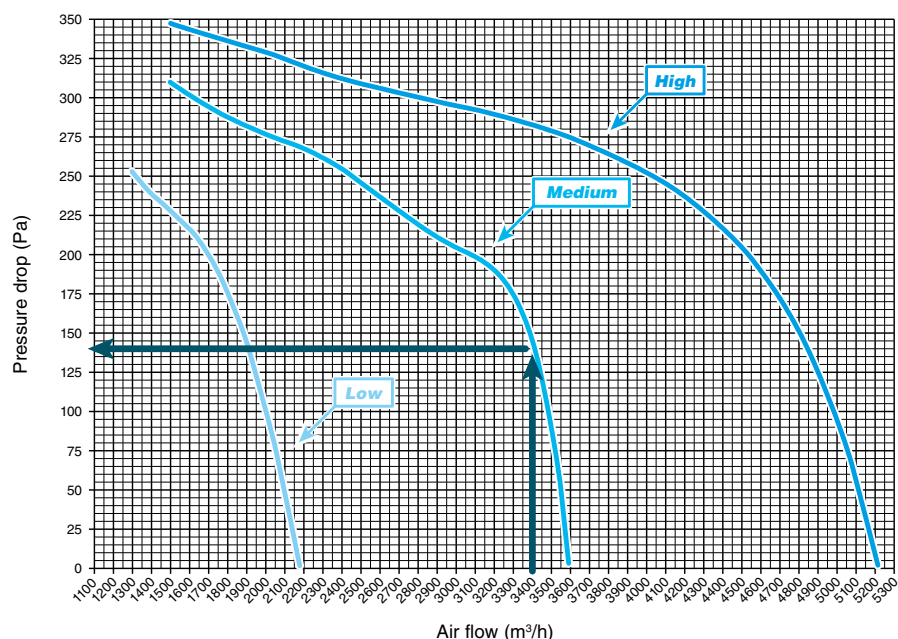
Diagram for Maestro MTL 64 “Available pressure”
